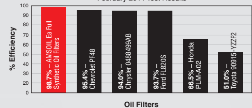
Average Filter Efficiency @ 20 Microns (ISO 4548-12)
